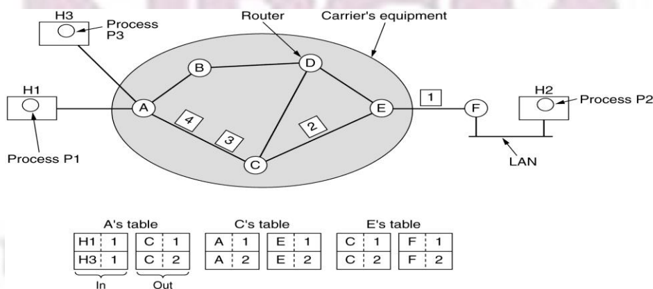
Fig: Routing within a virtual-circuit subnet
