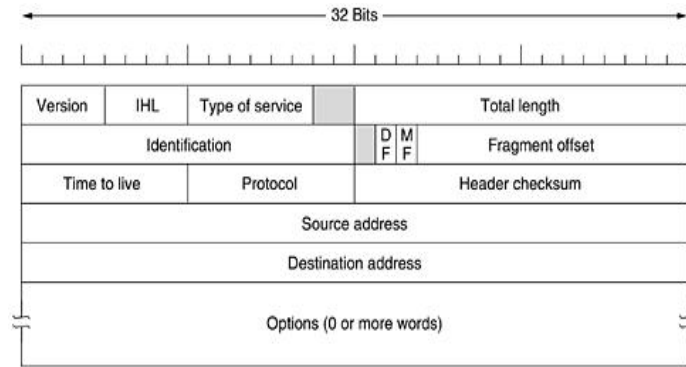
Fig: The IPv4 (Internet Protocol) header.
